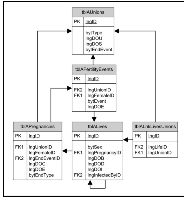
Figure 9: Entity Relationship Diagram for SPEHS 7
