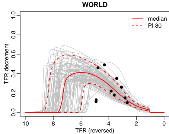
Figure 9: Projected trajectories for the world. Figure 10: Posterior distribution of the double logistic function for the world.
