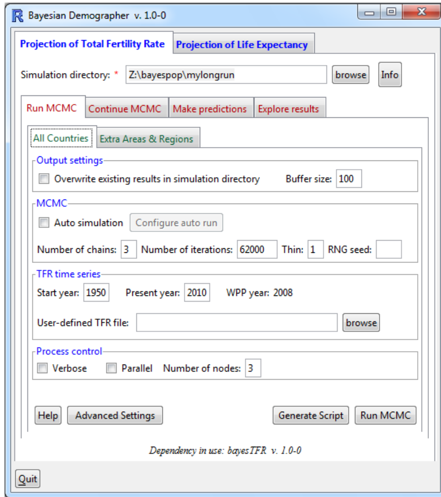
Figure 13: Graphical user interface for bayesTFR , implemented in the package bayesDem .
