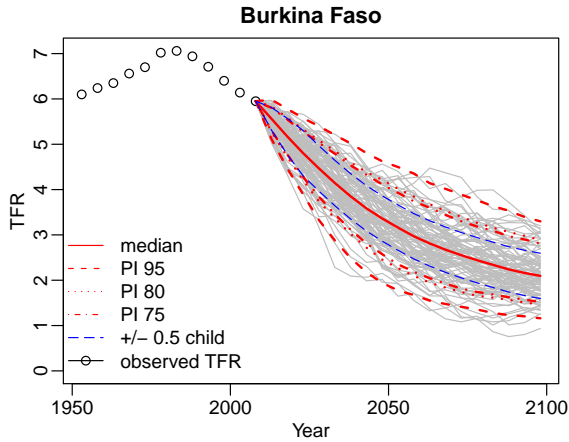
Figure 2: Projected trajectories for Burkina Faso.
