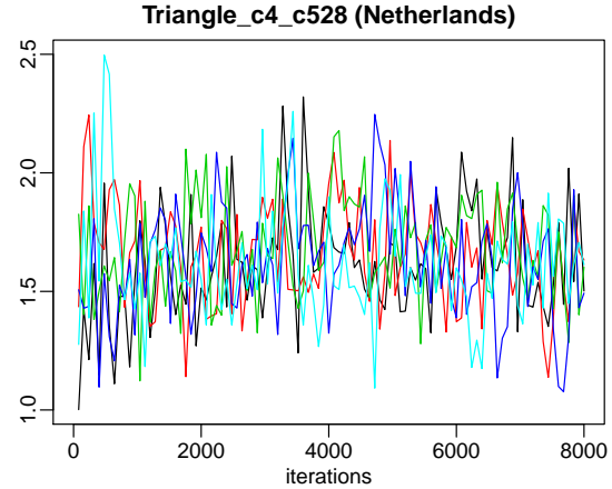
Figure 7: Parameter traces for the country-specific parameter \Delta_{c4} for the Netherlands, generated via the simulation in Section 3.1.
