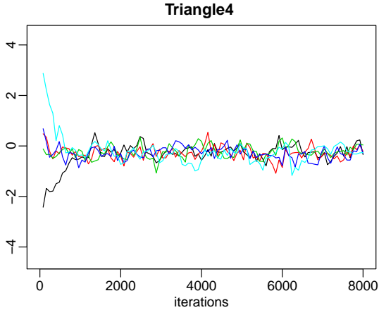
Figure 6: Parameter traces for the parameter \Delta_4 , generated via the simulation in Section 3.1.
