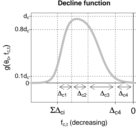
Figure 1: Five-year decrements as given by the double logistic decline function g(\boldsymbol{\theta}_c, f_{c,t}) plotted against the TFR. The horizontal TFR axis is negatively oriented (i.e. decreasing from left to right).
